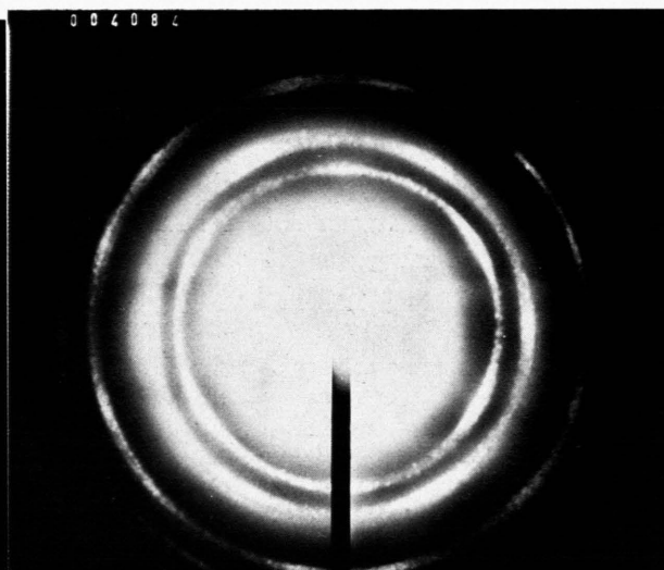
Fig. 3. Electron diffraction pattern taken from a specimen decorated at a substrate temperature of 900 °C.
